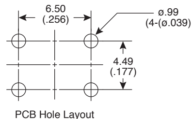
PCB Hole Layout
