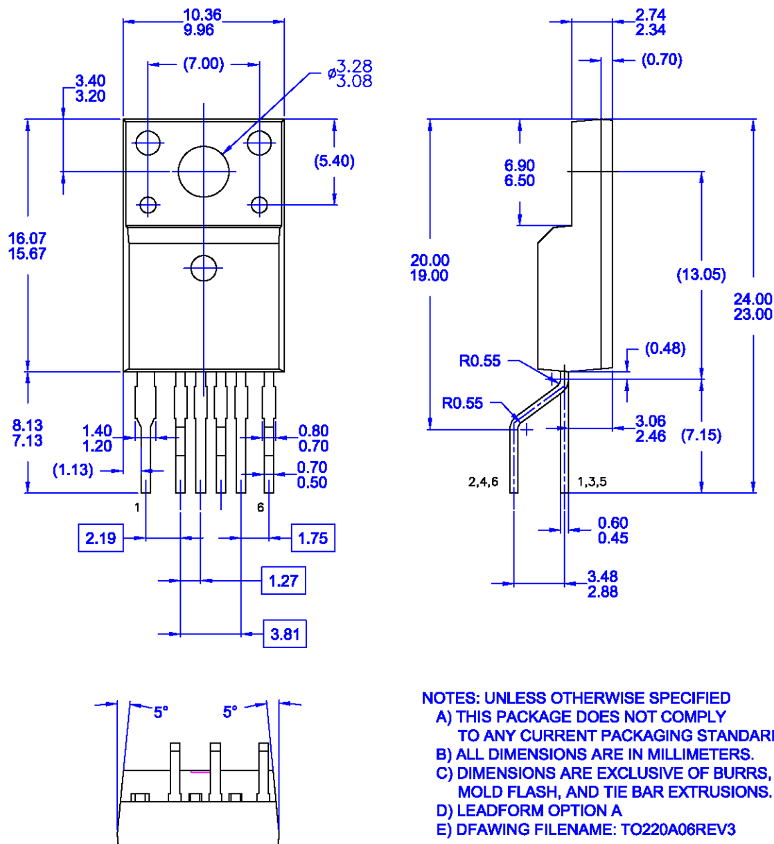
Figure 27. TO-220F-6L (Forming)
