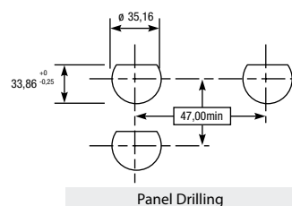
Panel Drilling
