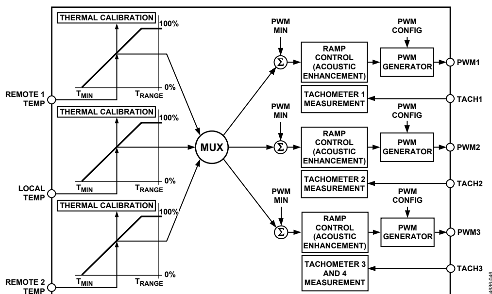
Figure 44. Automatic Fan Control Block Diagram
