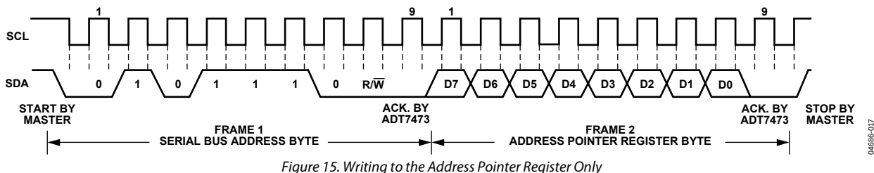
Figure 15. Writing to the Address Pointer Register Only
