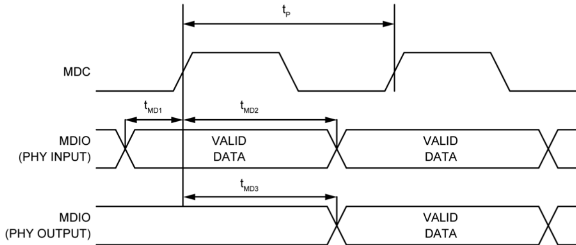
Figure 13. MDC/MDIO Timing
