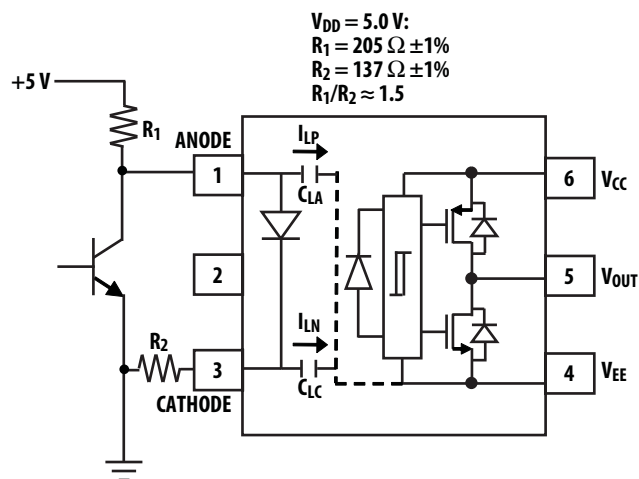
Figure 26. Recommended high-CMR drive circuit for the ACPL-P341/W341
