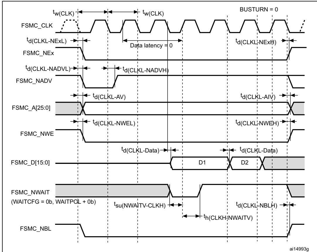
Figure 25. Synchronous non-multiplexed PSRAM write timings
