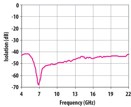
Figure 2. Isolation
