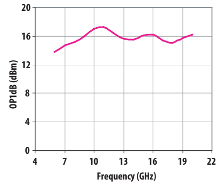
Figure 6. P1dB
