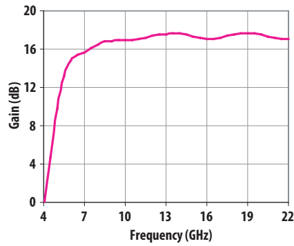
Figure 1. Gain
