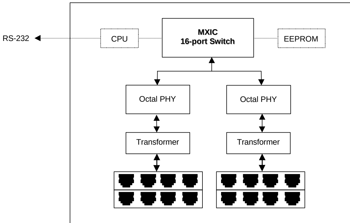
Figure 2. MX98216EC System Block Diagram
