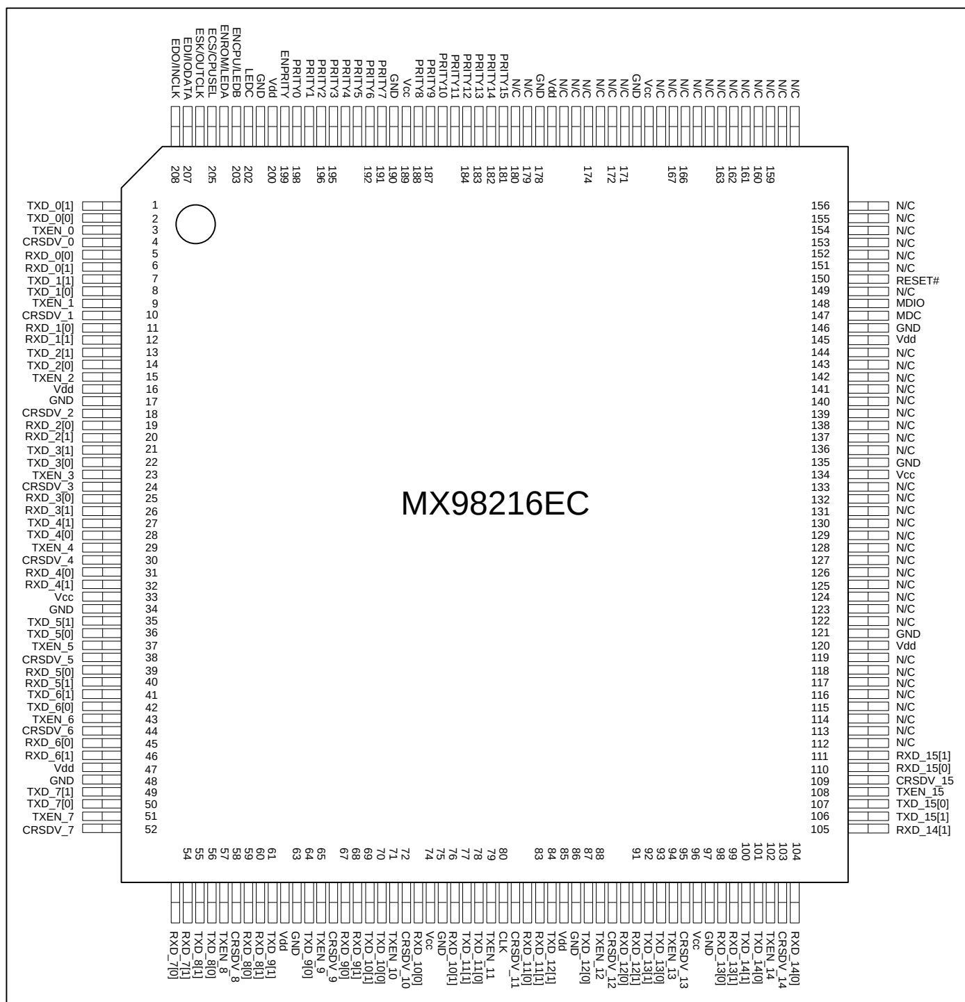
Figure 3. MX98216EC Pin Diagram Top View
