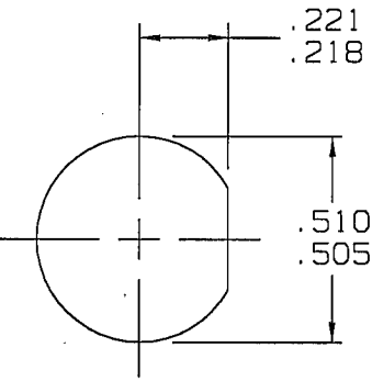
RECOMMENDED PANEL CUTOUT SCALE: 2/1
