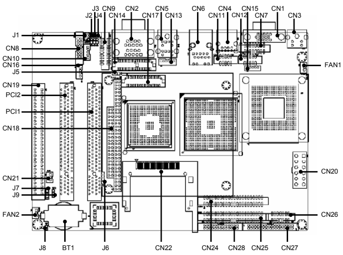
POD-6552 Connectors and Jumpers Location (Component side)
