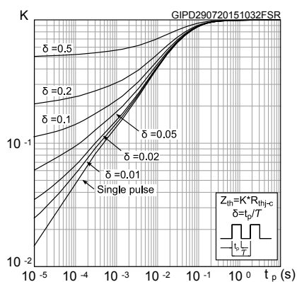
Figure 17. Thermal impedance
