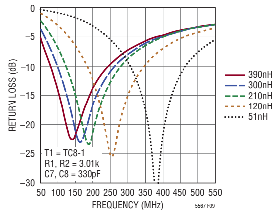
Figure 9. IF Output Return Loss—400Ω Bandpass Matching with 8:1 Transformer
