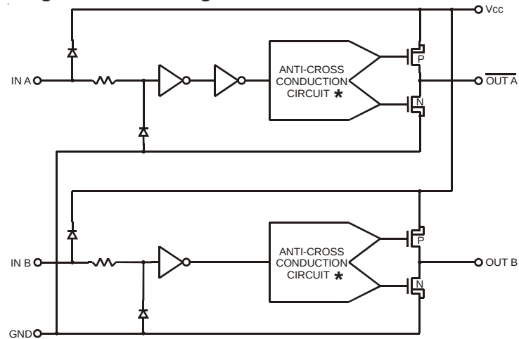
Figure 1 - IXDF504 Inverting + Non-Inverting 4A Gate Driver Functional Block Diagram
