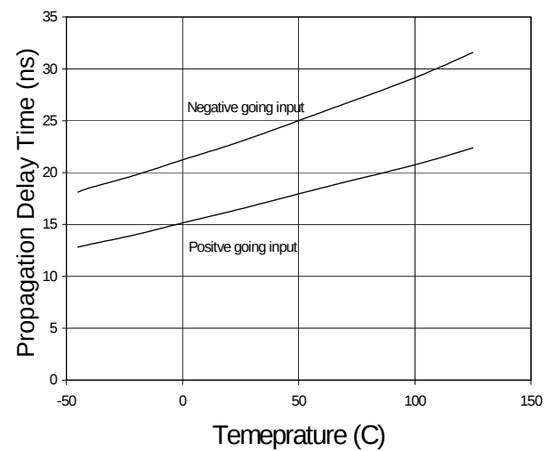
Fig. 14 Propagation Delay vs. Temperature V_{\text{SUPPLY}} = 15\text{V} C_{\text{LOAD}} = 1000\text{pF}
