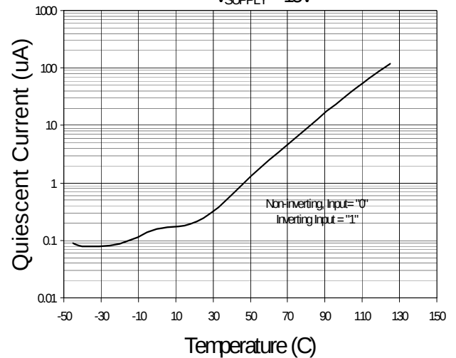
Fig. 16 Quiescent Current vs. Temperature V_{\text{SUPPLY}} = 15\text{V}
