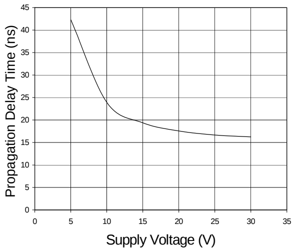
Fig. 13 Propagation Delay vs. Supply Voltage Falling Input, C_{\text{LOAD}} = 1000\text{pF}
