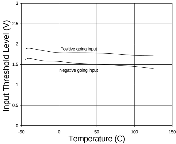
Fig. 11 Input Threshold Levels vs. Temperature V_{\text{SUPPLY}} = 15\text{V}
