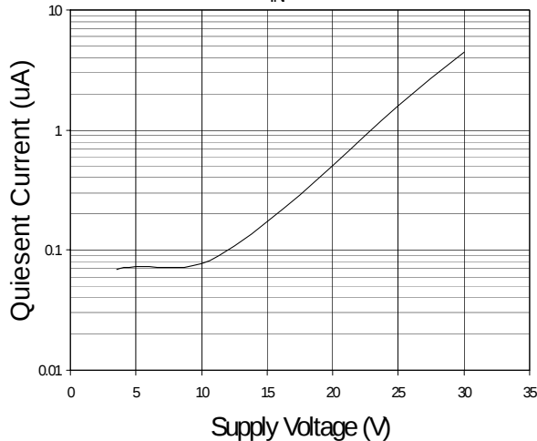
Fig. 15 Quiescent Current vs. Supply Voltage V_{\text{IN}} = 0\text{V}
