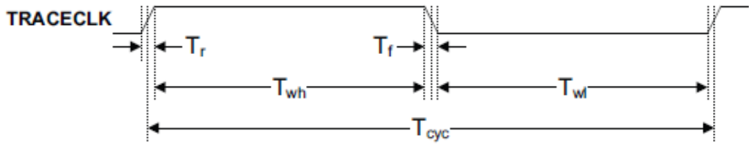
Figure 3. TRACE_CLKOUT specifications
