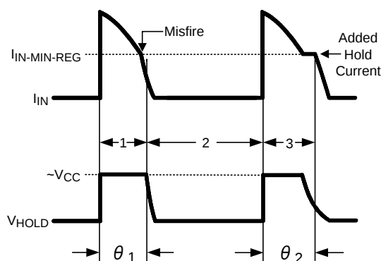
Figure 33. Dynamic Hold Waveform
