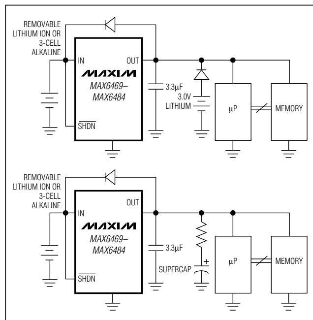
Figure 3. Battery Backup
