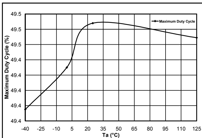
Maximum Duty Cycle vs. Temperature
