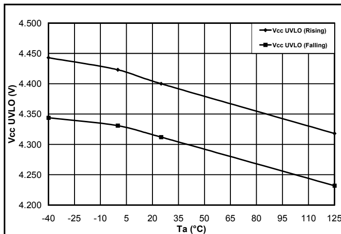
Vcc UVLO vs. Temperature
