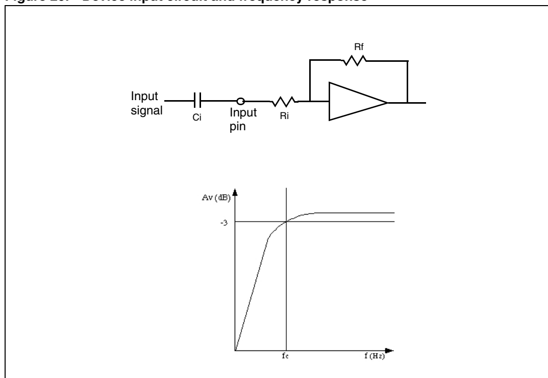
Figure 29. Device input circuit and frequency response
