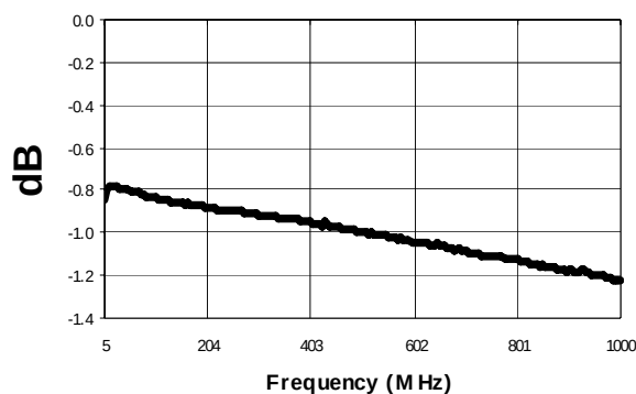
Mainline Loss
