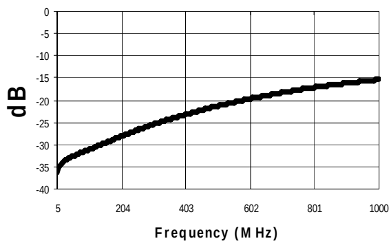
Directivity
