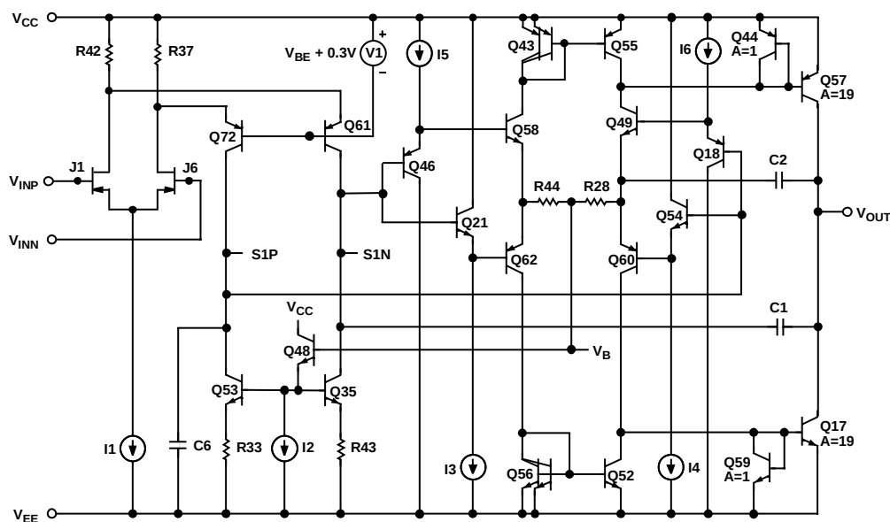
Figure 36. Simplified Schematic
