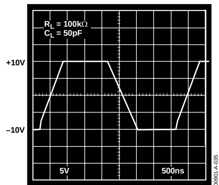
Figure 35. Pulse Response, V_S = \pm 15\text{ V} , G = +1
