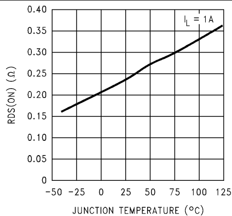
Figure 5-4. Drain-to-Source Resistance
