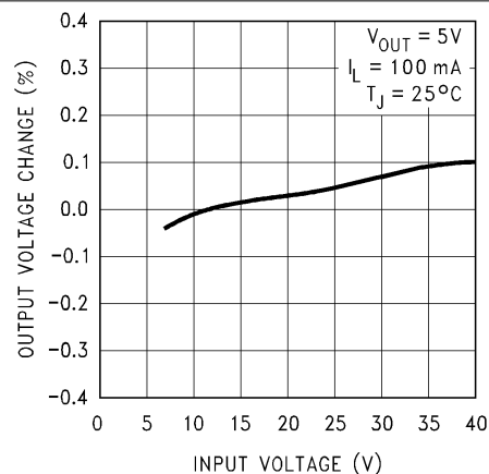
Figure 5-2. Line Regulation
