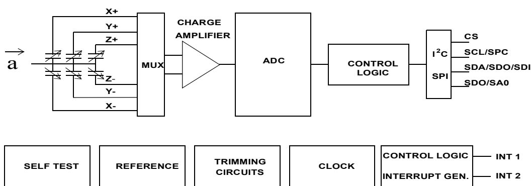
Figure 1. Block diagram
