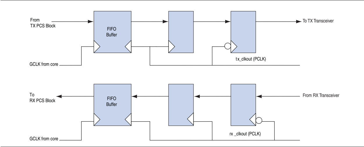
Figure 4-17. FIFO Buffer and Pipeline Registers Block
