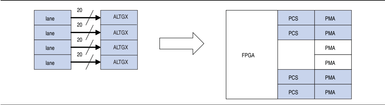
Figure 4-18. Transceiver Block Use in 4-, 8-, and 12-lane Variations
