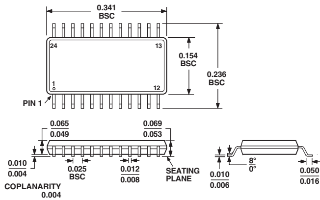
24-Lead Shrink Small Outline Package [QSOP] (RQ-24)
