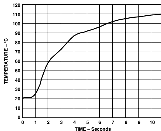
TPC 11. ADM1029 Response to Thermal Shock
