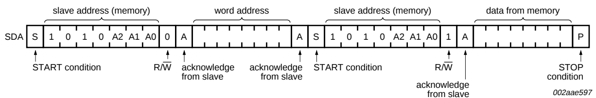
Fig 13. Random read
