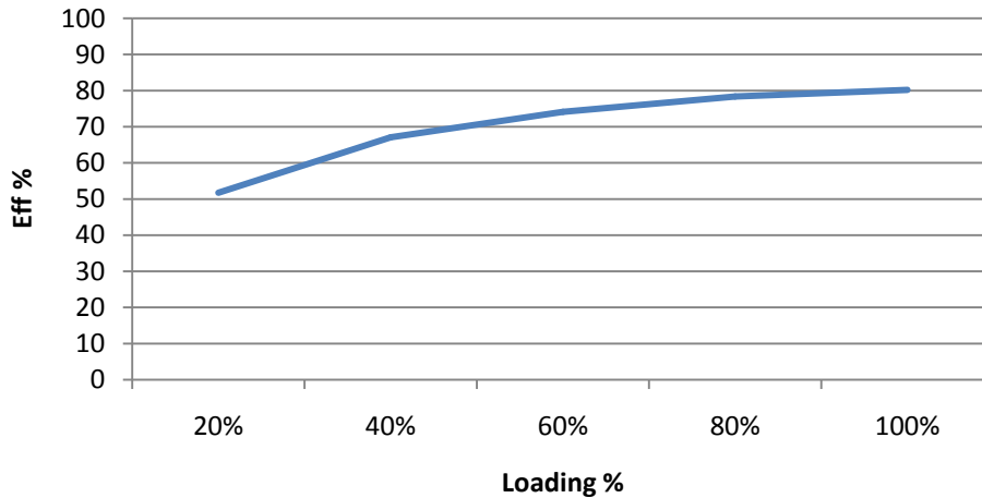
AM1S-4809SZ Efficiency vs. Loading
