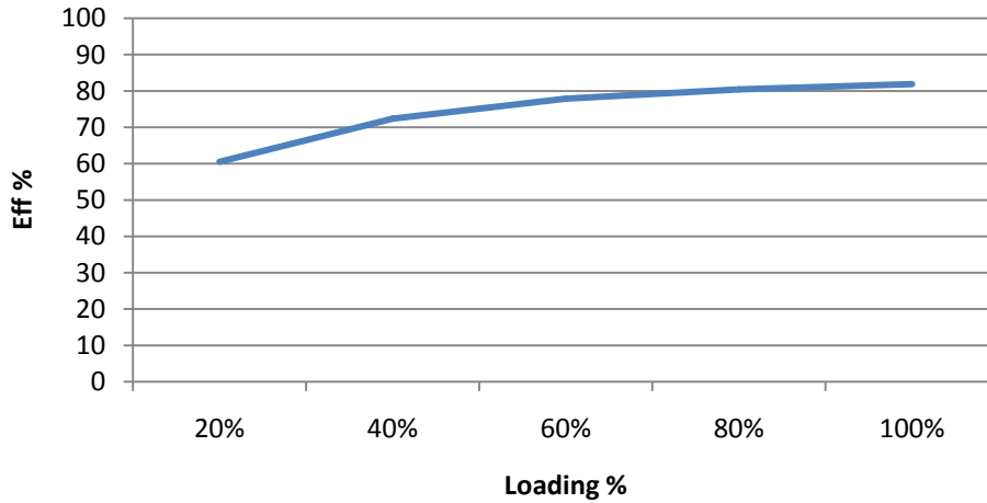
AM1S-2405SZ Efficiency vs. Loading
