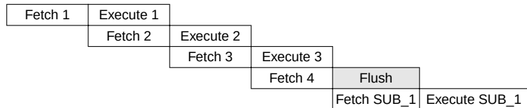
EXAMPLE 3-1: INSTRUCTION PIPELINE FLOW
