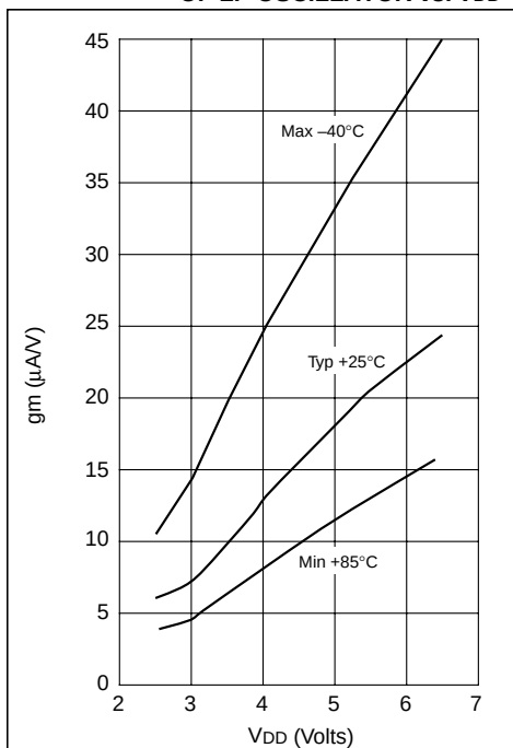
FIGURE 18-19: TRANSCONDUCTANCE (gm) OF XT OSCILLATOR vs. V DD
