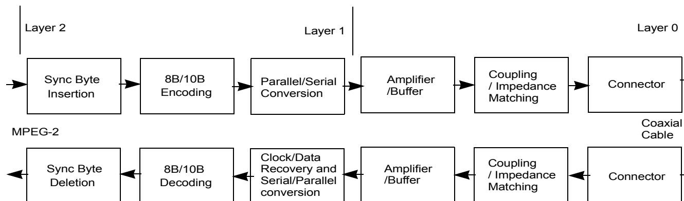
Figure 4-2.DVB-ASI Transmission Blocks
