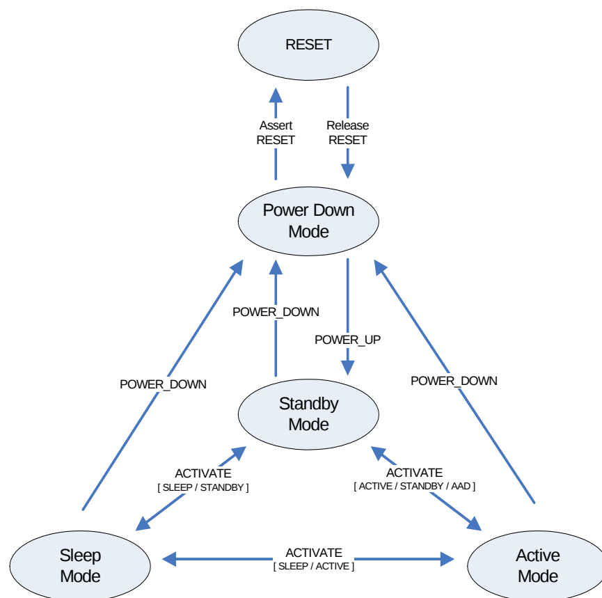
Figure 14. Operating Modes
