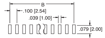
PH1RB-10-UA-SMT
