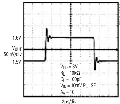
MAX4249/MAX4255/MAX4256/MAX4257 SMALL-SIGNAL PULSE RESPONSE
