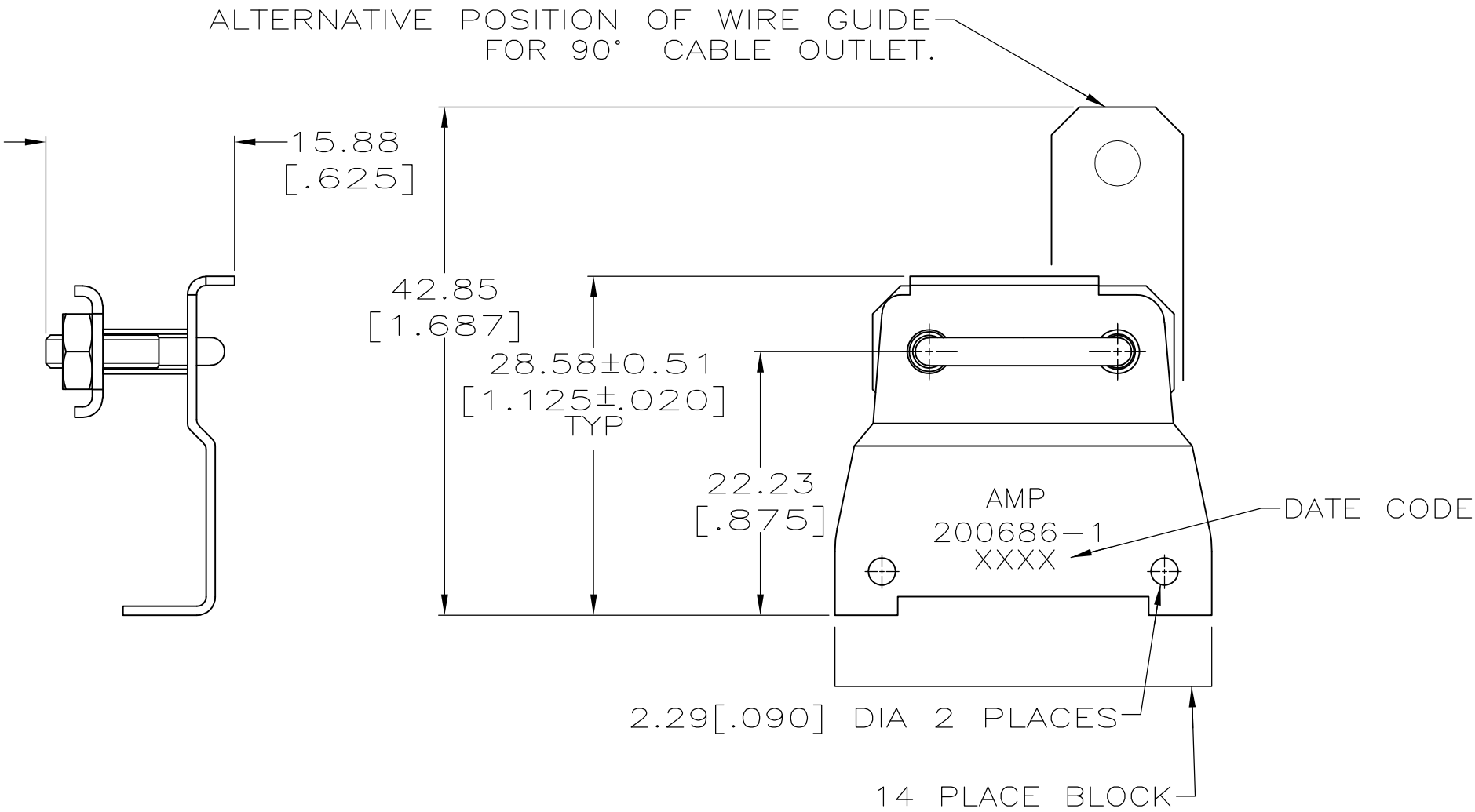
ASSEMBLED VIEW
