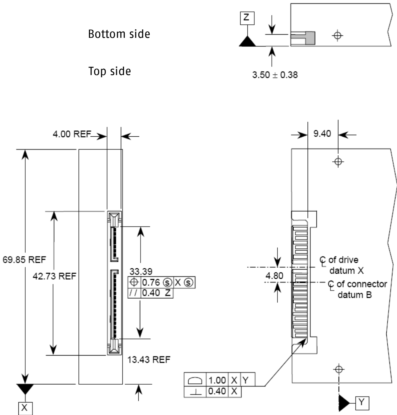
Figure 2: Connector location
