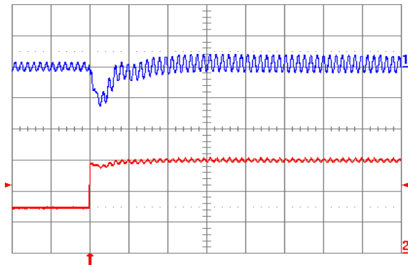
Fig. 1.8V.7: Output voltage response for V_{out} = 1.8 V to positive load current step change from 2.5 A to 5 A with slew rate of 5 A/ \mu\text{s} at V_{in} = 5 V. Top trace: output voltage (100 mV/div.); Bottom trace: load current (2 A/div.). C_o = 47 \mu\text{F} ceramic + 1 \mu\text{F} ceramic. Time scale: 20 \mu\text{s} /div.
