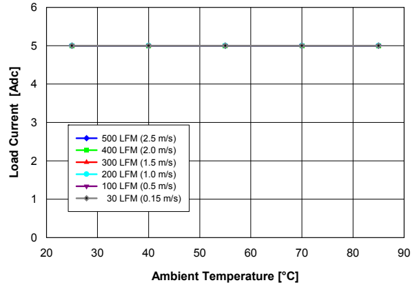
Fig. 2.5V.2: Available load current vs. ambient temperature and airflow rates for Vout = 2.5 V converter mounted horizontally with Vin = 5 V, air flowing from pin 5 to pin 1, and maximum MOSFET temperature ≤ 120 °C.
