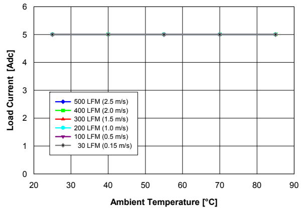
Fig. 0.7525V.2: Available load current vs. ambient temperature and airflow rates for Vout = 0.7525 V converter mounted horizontally with Vin = 5 V, air flowing from pin 5 to pin 1, and maximum MOSFET temperature ≤ 120 °C.
