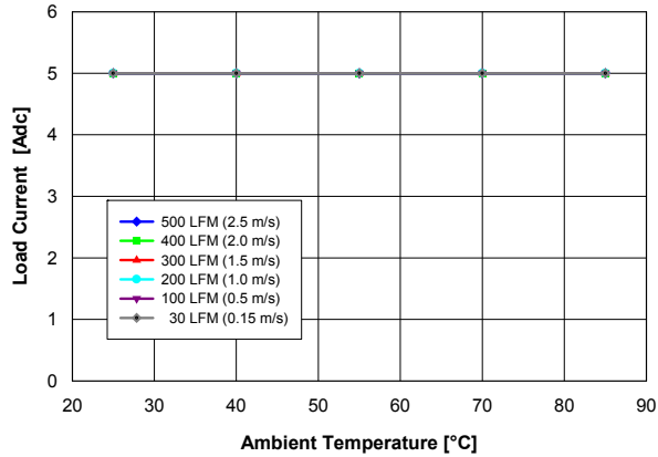
Fig. 1.8V.1: Available load current vs. ambient temperature and airflow rates for V_{out} = 1.8 V converter mounted vertically with V_{in} = 5 V, air flowing from pin 5 to pin 1, and maximum MOSFET temperature \leq 120 °C.
