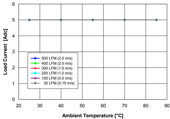
Fig. 2.5V.1: Available load current vs. ambient temperature and airflow rates for Vout = 2.5 V converter mounted vertically with Vin = 5 V, air flowing from pin 5 to pin 1, and maximum MOSFET temperature ≤ 120 °C.
