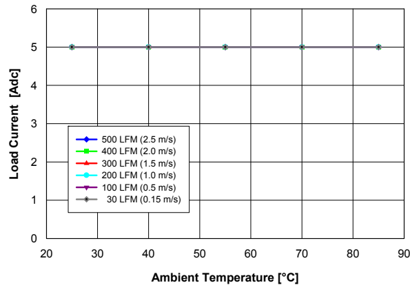
Fig. 2.0V.1: Available load current vs. ambient temperature and airflow rates for Vout = 2.0 V converter mounted vertically with Vin = 5 V, air flowing from pin 5 to pin 1, and maximum MOSFET temperature ≤ 120 °C.
