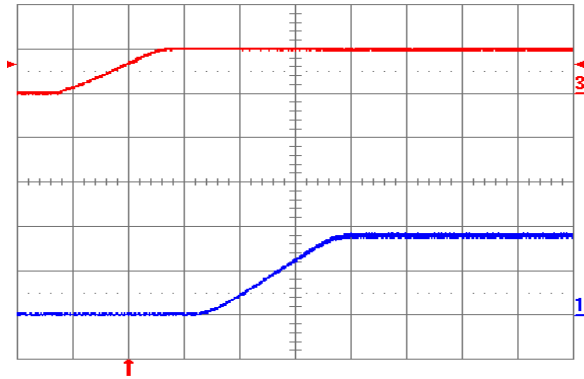
Fig. 1.8V.5: Turn-on transient for V_{out} = 1.8 V with application of V_{in} at full rated load current (resistive) and 47 \mu\text{F} external capacitance at V_{in} = 5 V. Top trace: V_{in} (5 V/div.); Bottom trace: output voltage (1 V/div.); Time scale: 2 ms/div.
