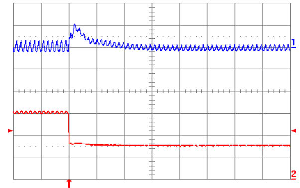
Fig. 1.2V.8: Output voltage response for V_{out} = 1.2 V to negative load current step change from 5 A to 2.5 A with slew rate of -5 \text{ A}/\mu\text{s} at V_{in} = 5 V. Top trace: output voltage (100 mV/div.); Bottom trace: load current (2 A/div.). C_o = 47 \mu\text{F} ceramic + 1 \mu\text{F} ceramic. Time scale: 20 \mu\text{s} /div.
