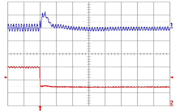
Fig. 1.8V.8: Output voltage response for V_{out} = 1.8 V to negative load current step change from 5 A to 2.5 A with slew rate of -5 A/ \mu\text{s} at V_{in} = 5 V. Top trace: output voltage (100 mV/div.); Bottom trace: load current (2 A/div.). C_o = 47 \mu\text{F} ceramic + 1 \mu\text{F} ceramic. Time scale: 20 \mu\text{s} /div.
