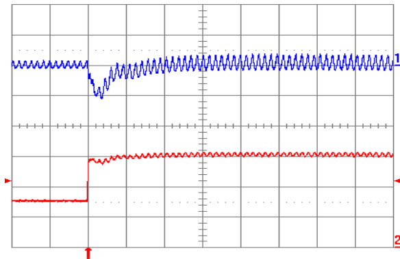
Fig. 1.2V.7: Output voltage response for V_{out} = 1.2 V to positive load current step change from 2.5 A to 5 A with slew rate of 5 \text{ A}/\mu\text{s} at V_{in} = 5 V. Top trace: output voltage (100 mV/div.); Bottom trace: load current (2 A/div.). C_o = 47 \mu\text{F} ceramic + 1 \mu\text{F} ceramic. Time scale: 20 \mu\text{s} /div.
