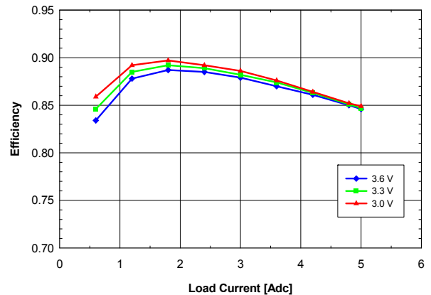
Fig. 1.0V.4: Efficiency vs. load current and input voltage for V_{out} = 1.0 V converter mounted vertically with air flowing from pin 5 to pin 1 at a rate of 200 LFM (1m/s) and T_a = 25 °C.
