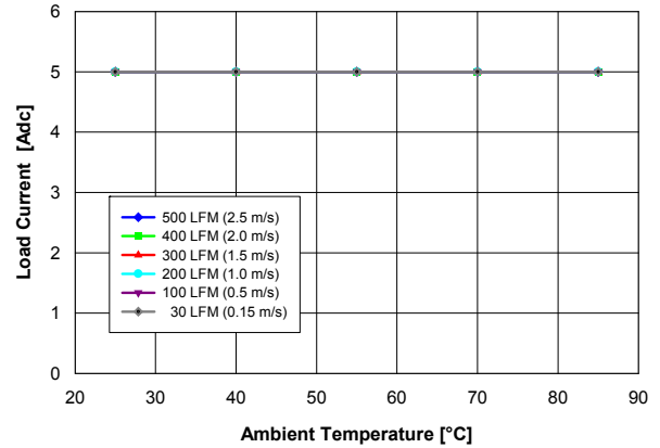
Fig. 1.8V.2: Available load current vs. ambient temperature and airflow rates for V_{out} = 1.8 V converter mounted horizontally with V_{in} = 5 V, air flowing from pin 5 to pin 1, and maximum MOSFET temperature \leq 120 °C.
