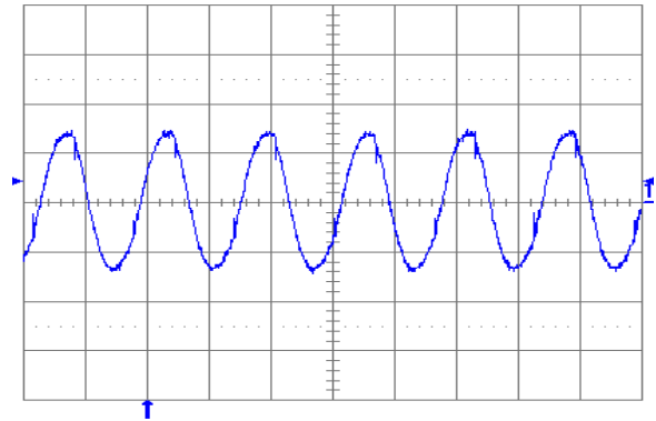
Fig. 1.8V.6: Output voltage ripple (20 mV/div.) at full rated load current into a resistive load with external capacitance 10 \mu\text{F} ceramic + 1 \mu\text{F} ceramic and V_{in} = 5 V for V_{out} = 1.8 V. Time scale: 2 \mu\text{s} /div.
