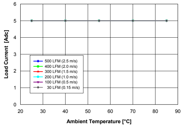
Fig. 0.7525V.1: Available load current vs. ambient temperature and airflow rates for Vout = 0.7525 V converter mounted vertically with Vin = 5 V, air flowing from pin 5 to pin 1, and maximum MOSFET temperature ≤ 120 °C.
