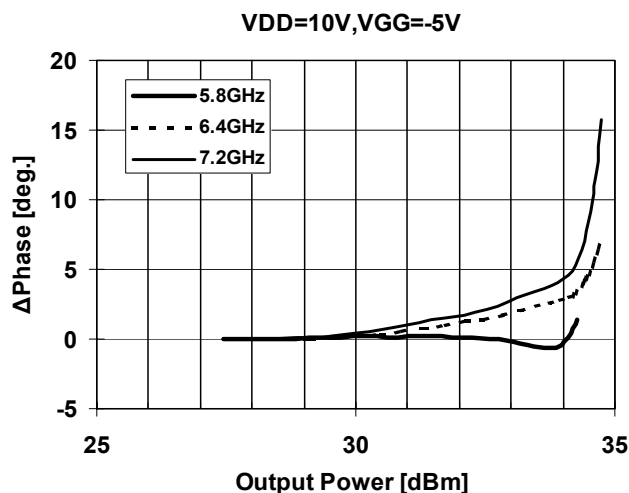
AMPM vs OUTPUT POWER
