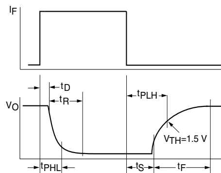
Figure 6. Switching Waveform
