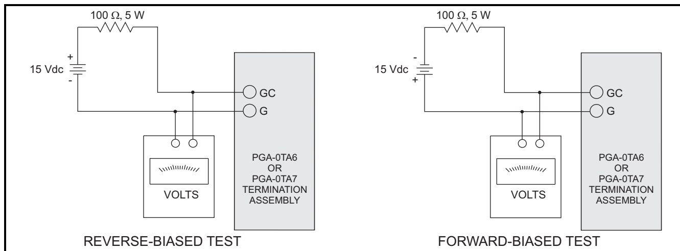
FIGURE 8. Termination-Assembly-Test Circuits.
