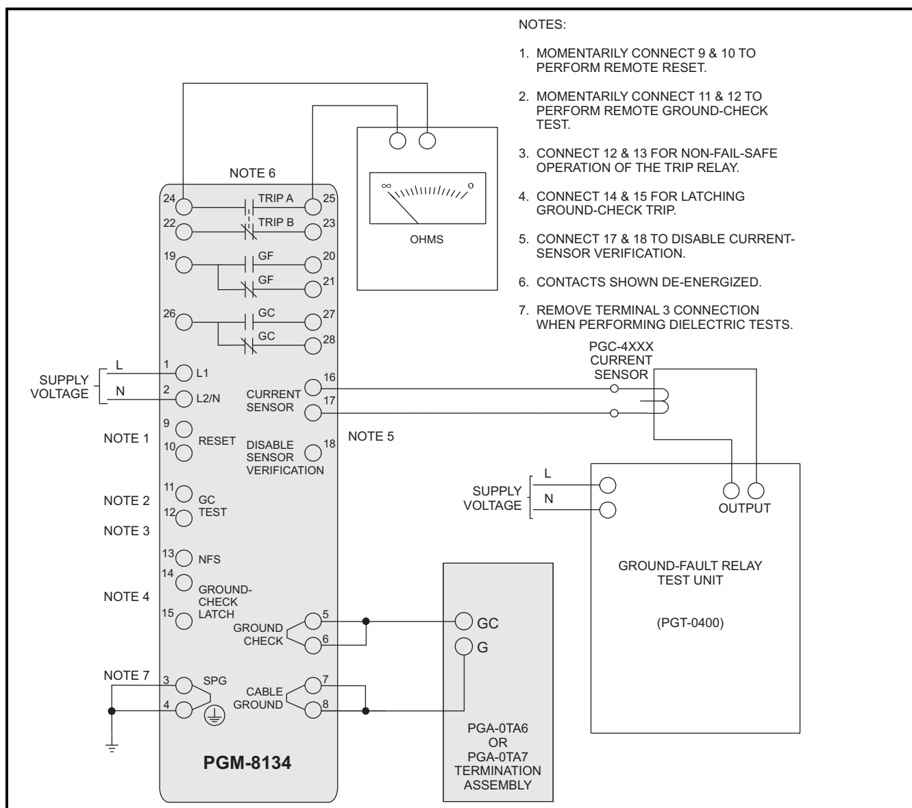
FIGURE 7. Ground-Fault-Test Circuit.
