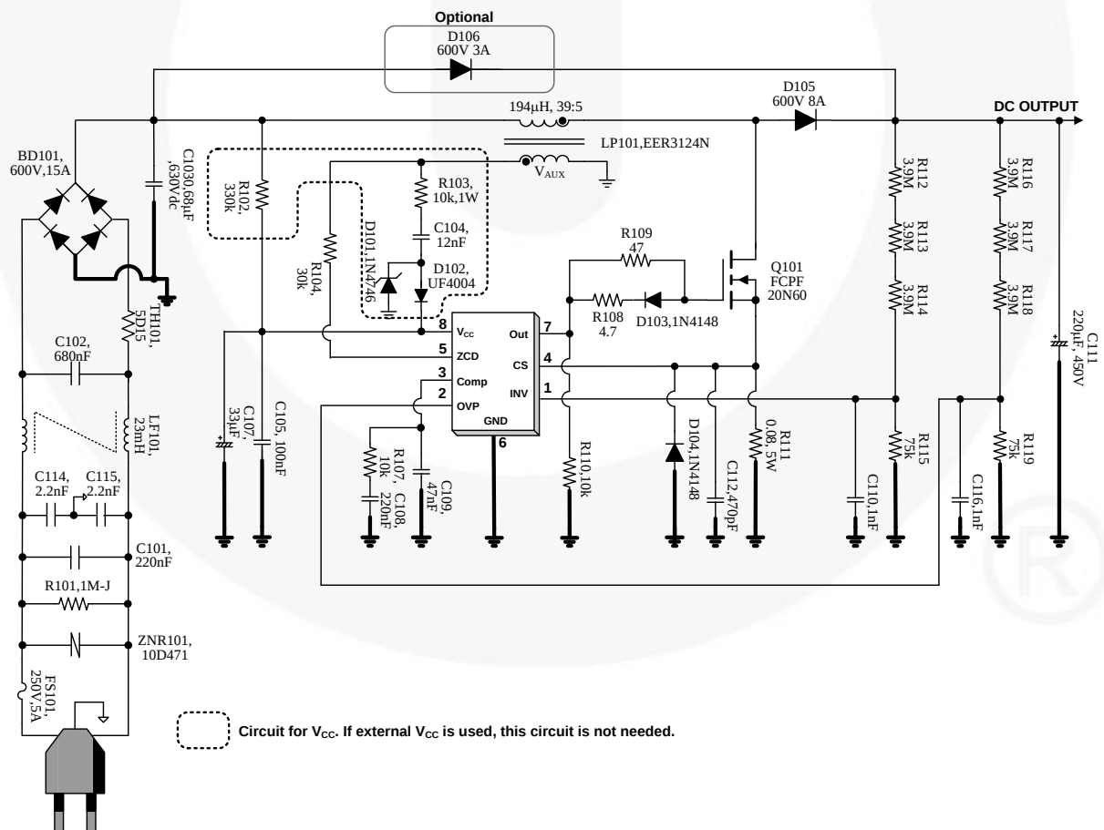
Figure 45. Demonstration Circuit
