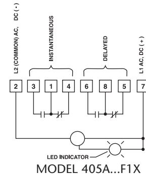
MODEL 405A...F1X
