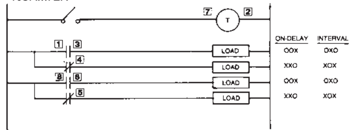
405A...F2X
