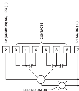
MODEL 405A...F2X
