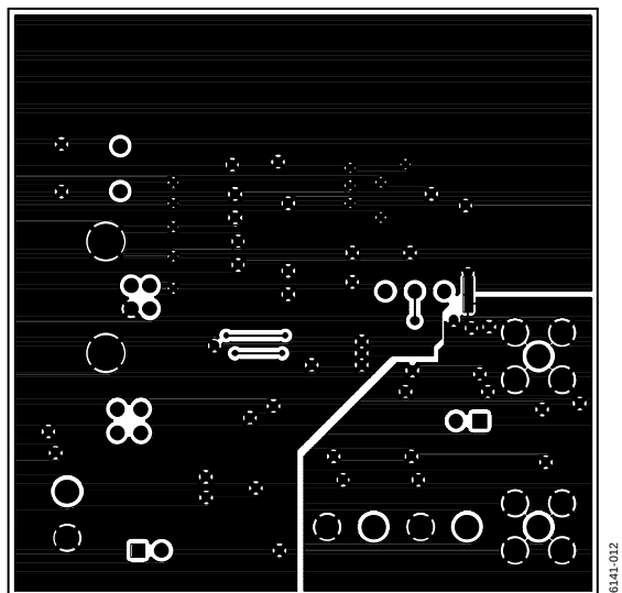
Figure 8. EVAL-AD5040EB/AD5060EB/AD5061EB/AD5062EB— Solder-Side Artwork
