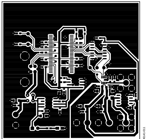
Figure 7. EVAL-AD5040EB/AD5060EB/AD5061EB/AD5062EB— Component Side Artwork
