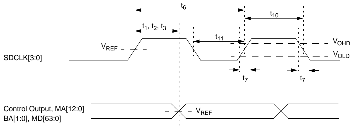
Figure 8-4. Output Valid Timing
