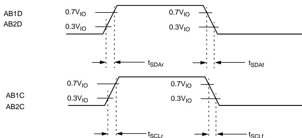
Figure 8-6. ACB Signals Rising Time and Falling Times
