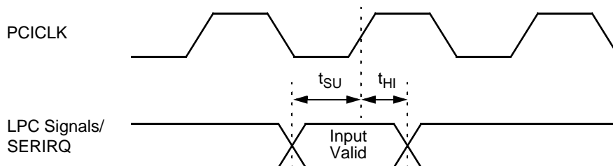
Figure 8-20. LPC Input Timing
