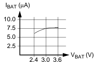
Figure 5-10. Typical Battery Current: Battery Backed Power Mode
