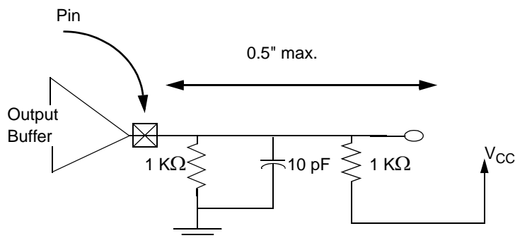
Figure 8-10. Testing Setup for Slew Rate and Minimum Timing
