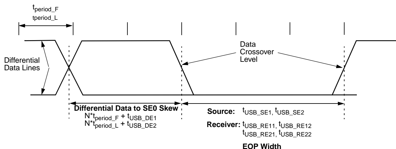
Figure 8-37. EOP Width Timing
