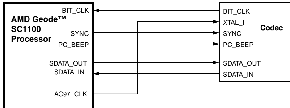
Figure 6-13. AC97 v2.0 Codec Signal Connections
