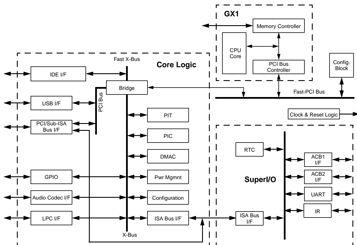
Figure 1-1. Block Diagram
