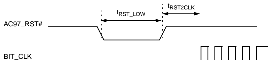
Figure 8-41. AC97 Reset Timing
