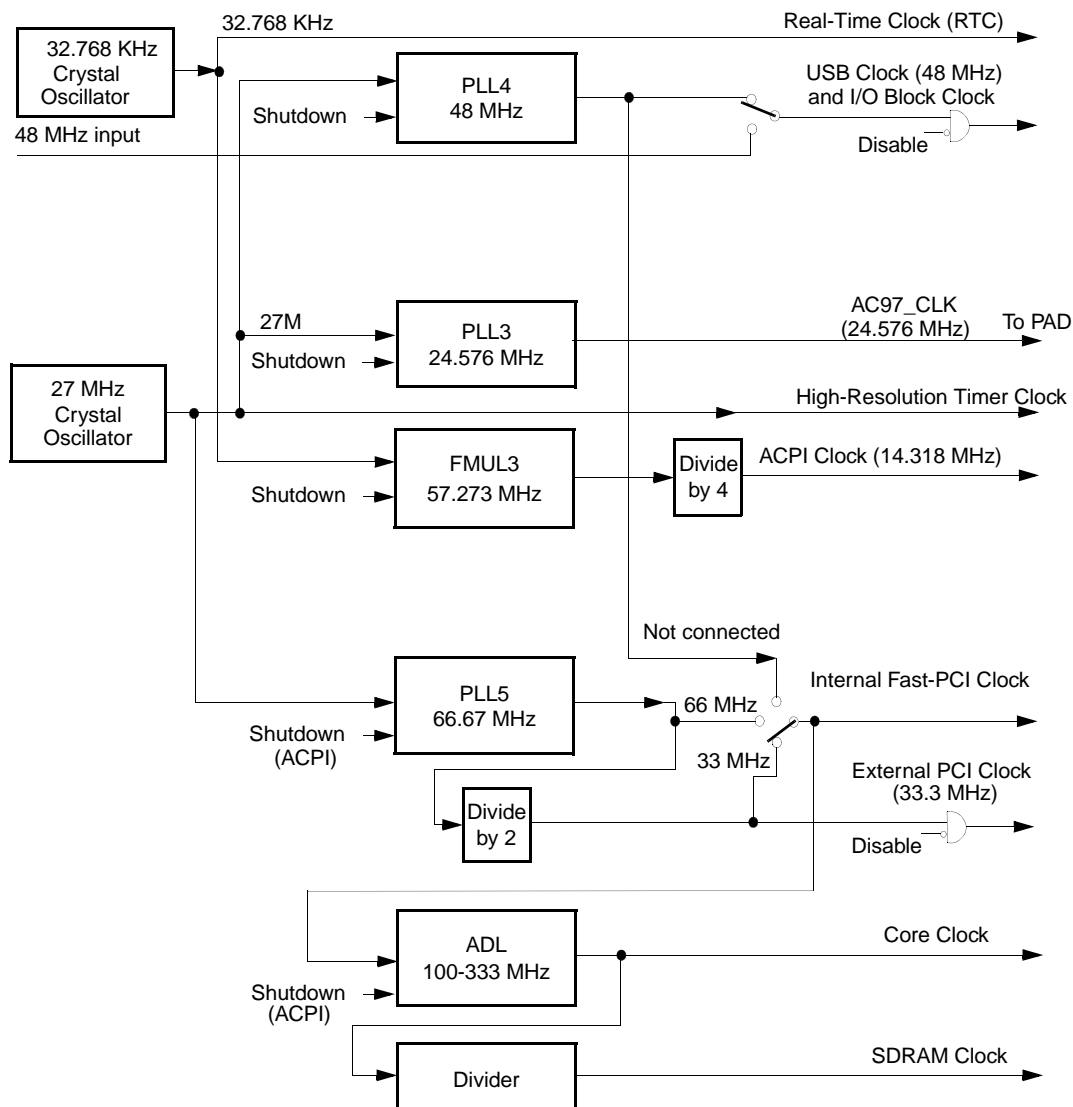
Figure 4-2. Clock Generation Block Diagram
