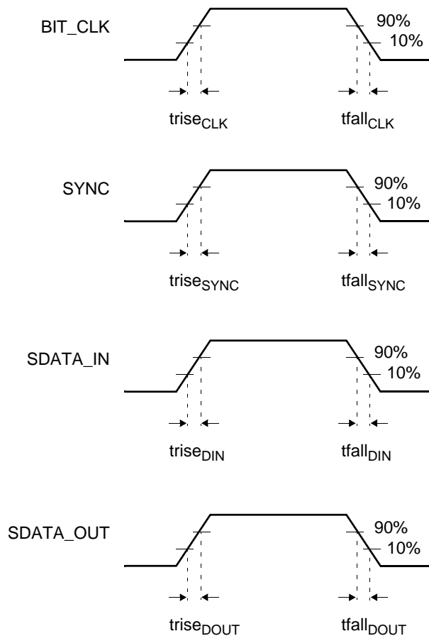
Figure 8-45. Rise and Fall Times
