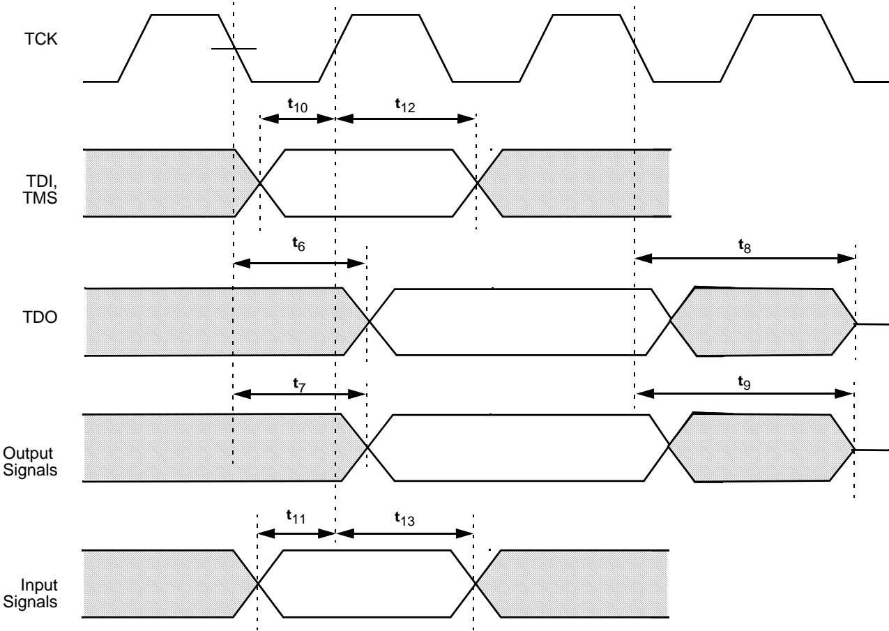
Figure 8-52. JTAG Test Timings
