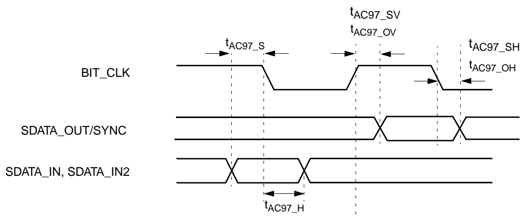
Figure 8-44. AC97 Data Timing
