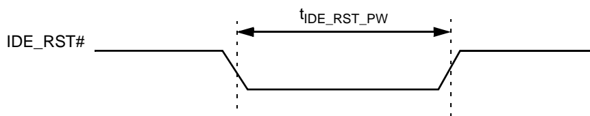
Figure 8-21. IDE Reset Timing
