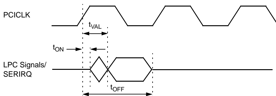
Figure 8-19. LPC Output Timing
