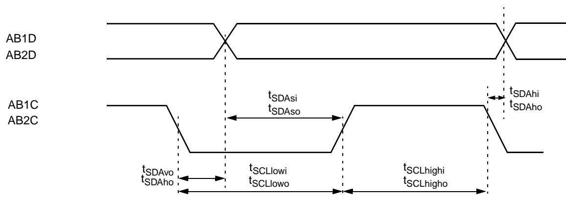
Figure 8-9. ACB Data Bit Timing
