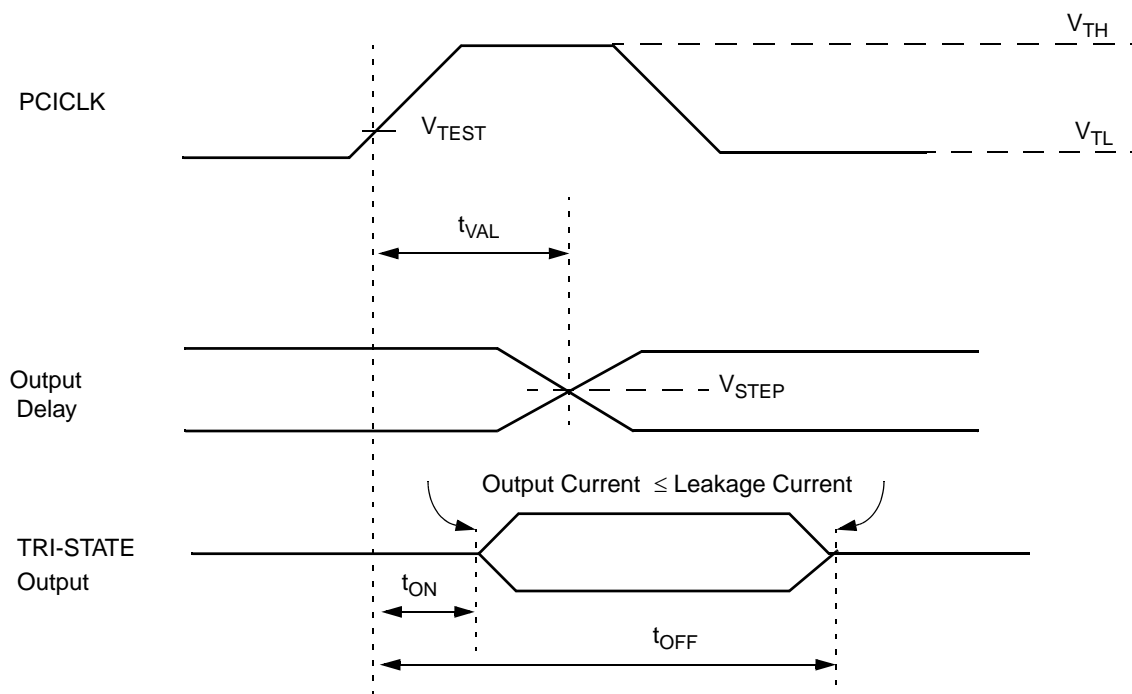
Figure 8-14. Output Timing Measurement Conditions
