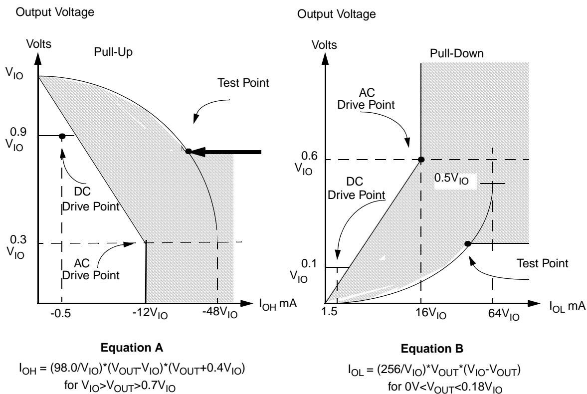
Figure 8-11. V/I Curves for PCI Output Signals
