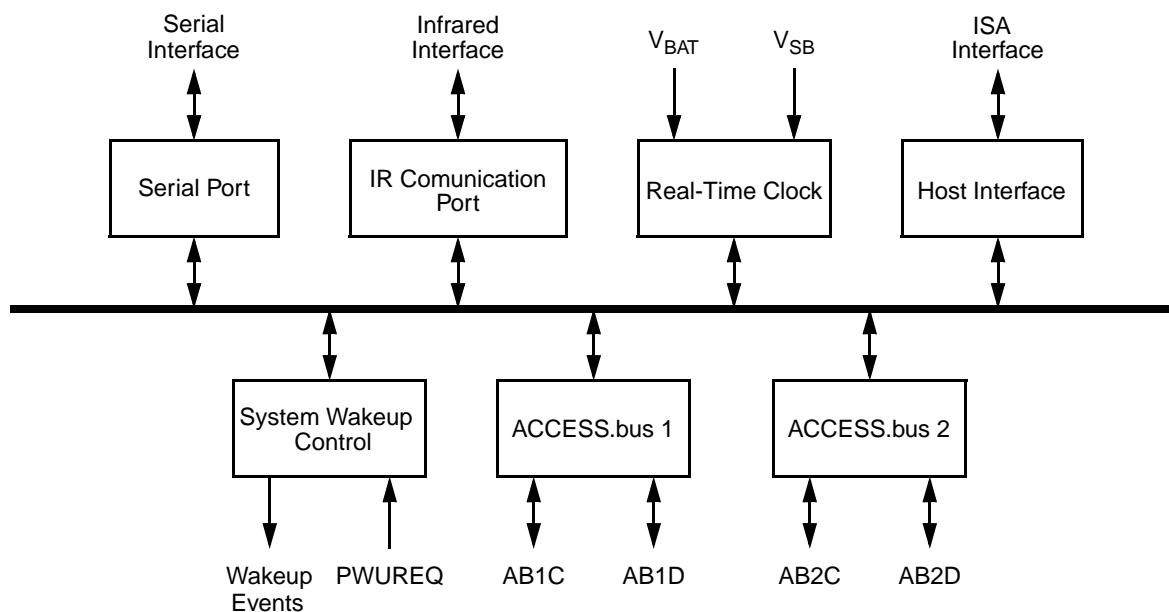
Figure 5-1. SIO Block Diagram
