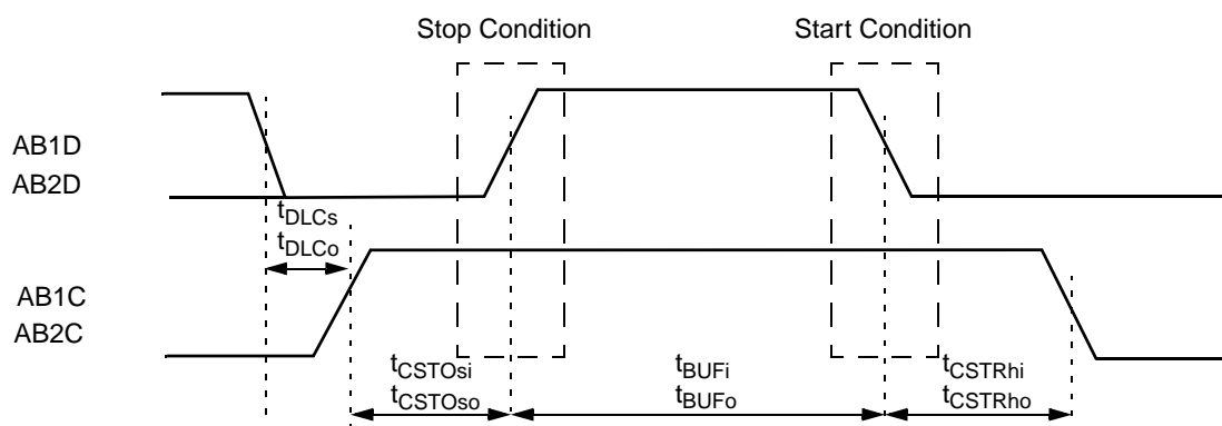
Figure 8-7. ACB Start and Stop Condition Timing
