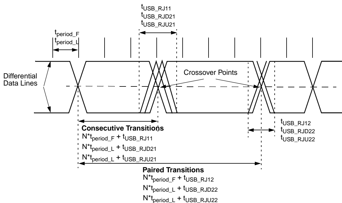
Figure 8-38. Receiver Jitter Tolerance
