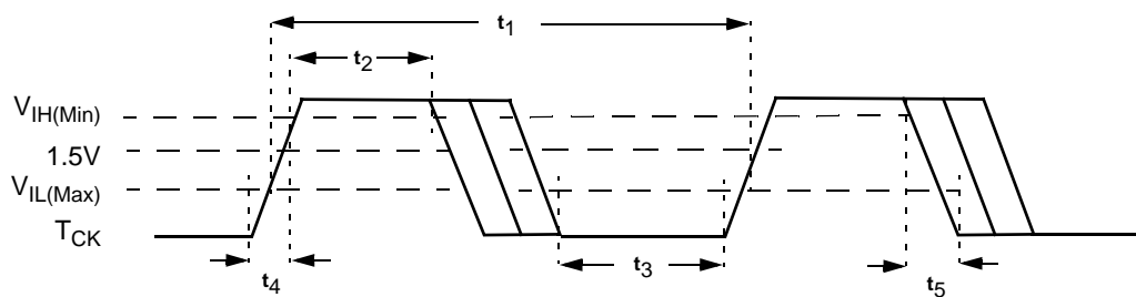
Figure 8-51. TCK Timing and Measurement Points
