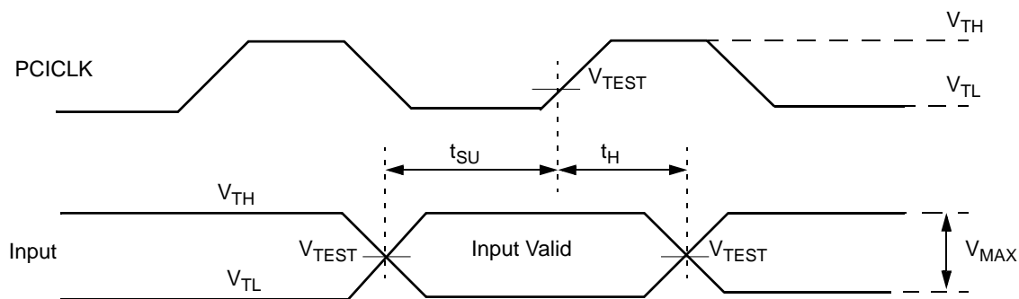
Figure 8-15. Input Timing Measurement Conditions
