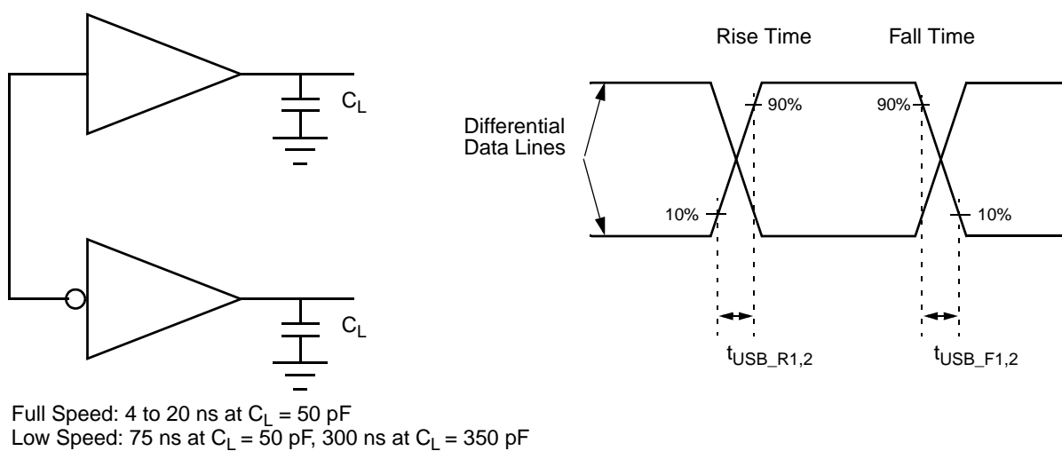
Figure 8-35. Data Signal Rise and Fall Time
