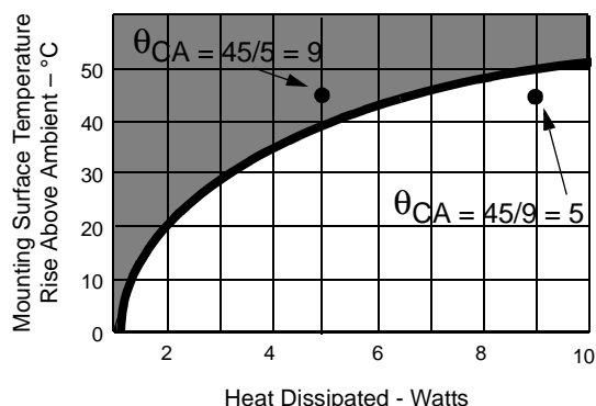
Figure 9-1. Heatsink Example
