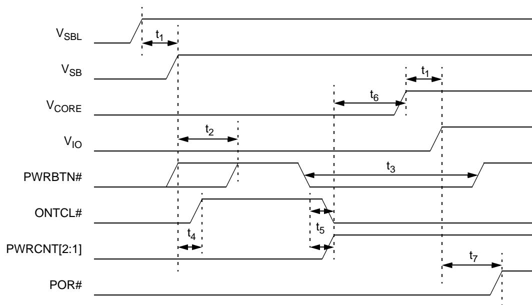
Figure 8-49. Power-Up Sequencing Timing
