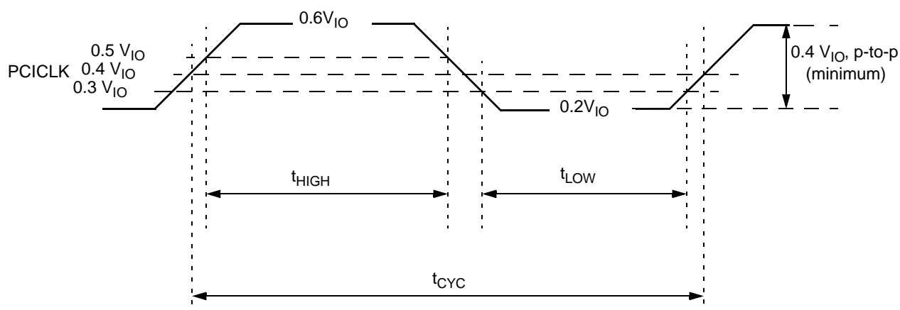
Figure 8-12. PCICLK Timing and Measurement Points
