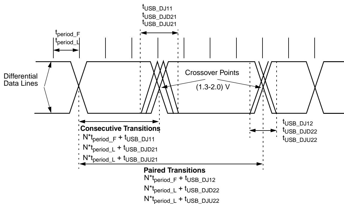
Figure 8-36. Source Differential Data Jitter
