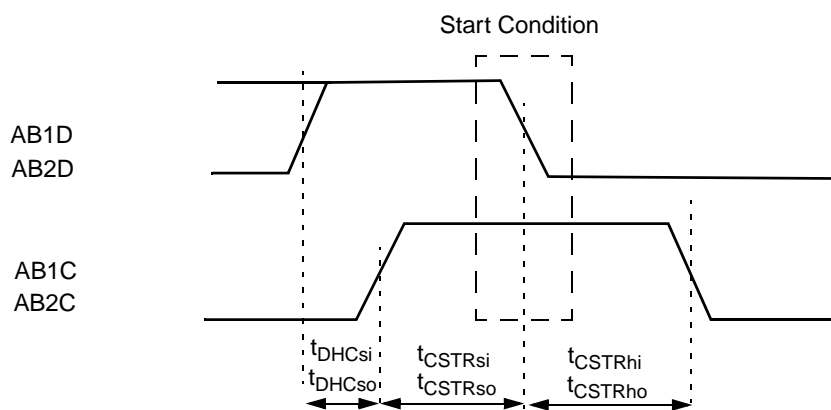
Figure 8-8. ACB Start Condition Timing
