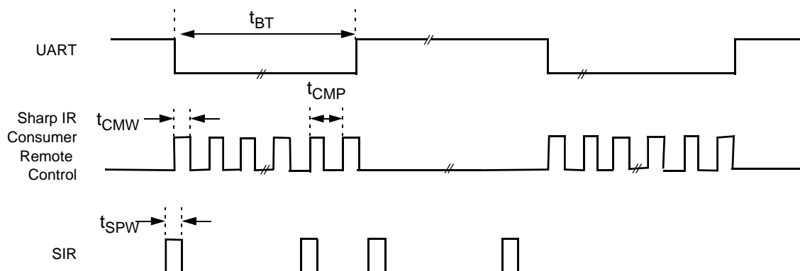
Figure 8-39. UART, Sharp-IR, SIR, and Consumer Remote Control Timing
