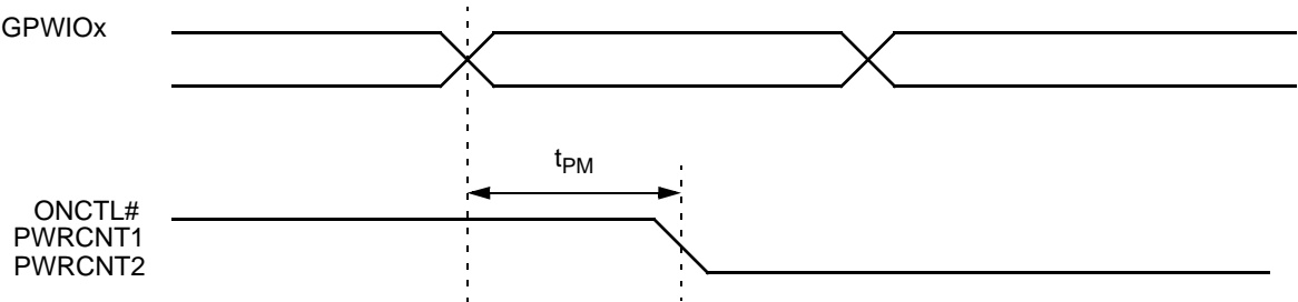
Figure 8-48. GPWIO and ONCTL# Timing
