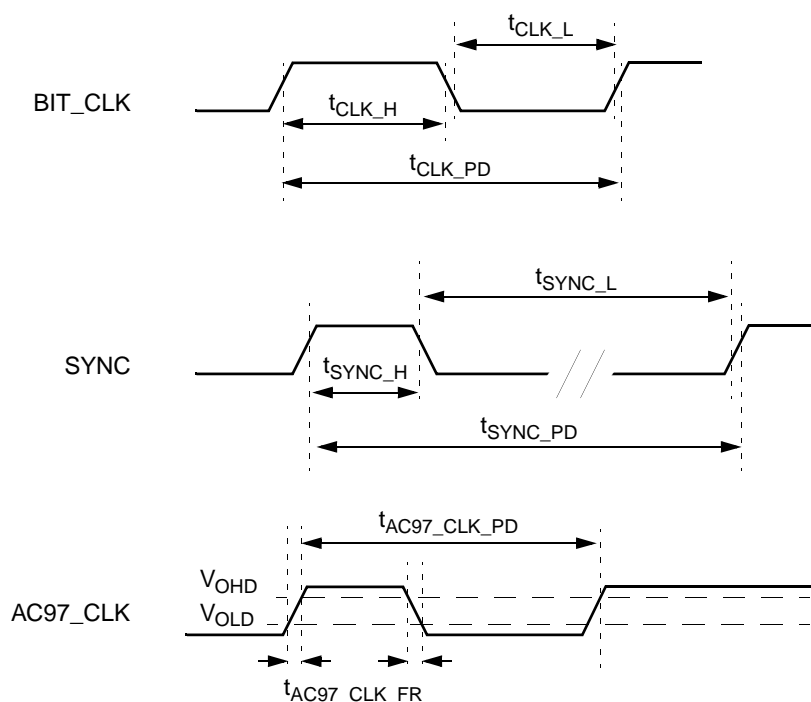
Figure 8-43. AC97 Clocks
