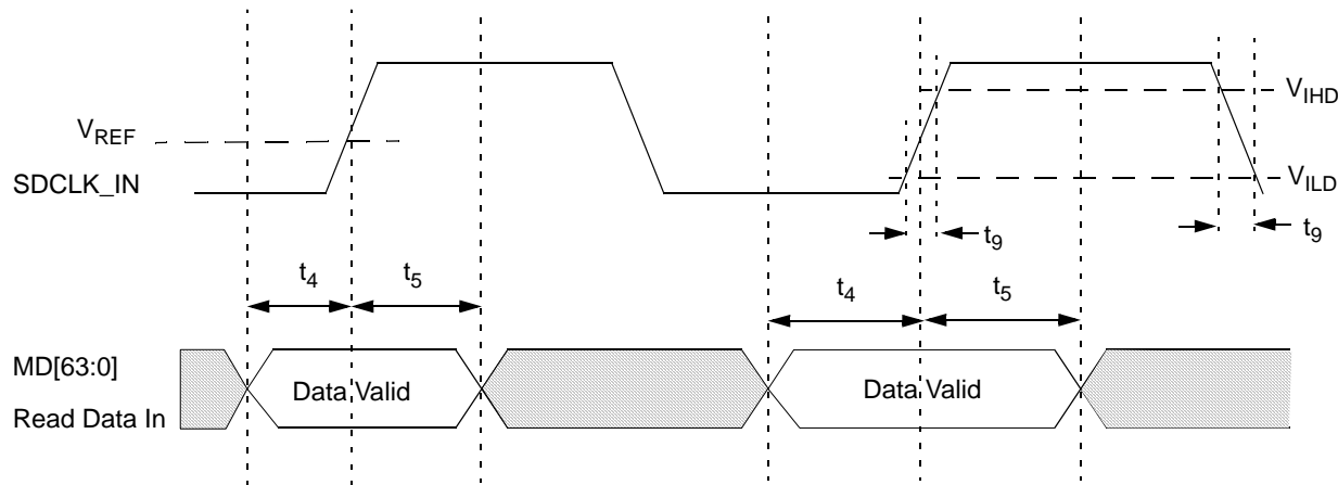
Figure 8-5. Setup and Hold Timing - Read Data In
