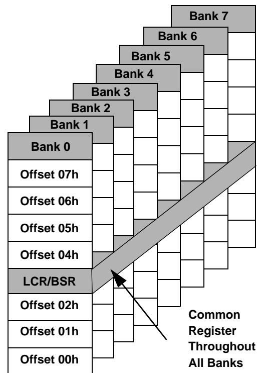
Figure 5-19. IRCP Register Bank Architecture
