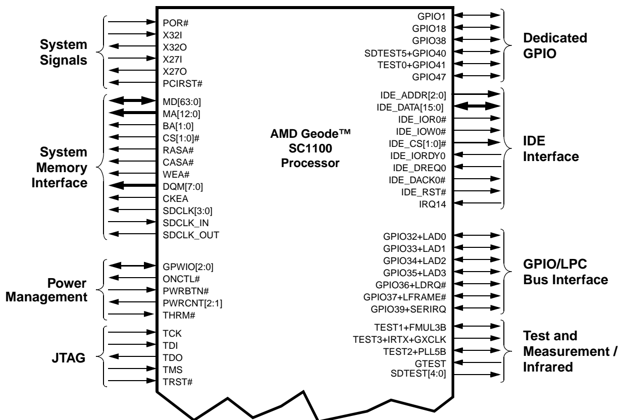
Figure 3-1. Signal Groups
