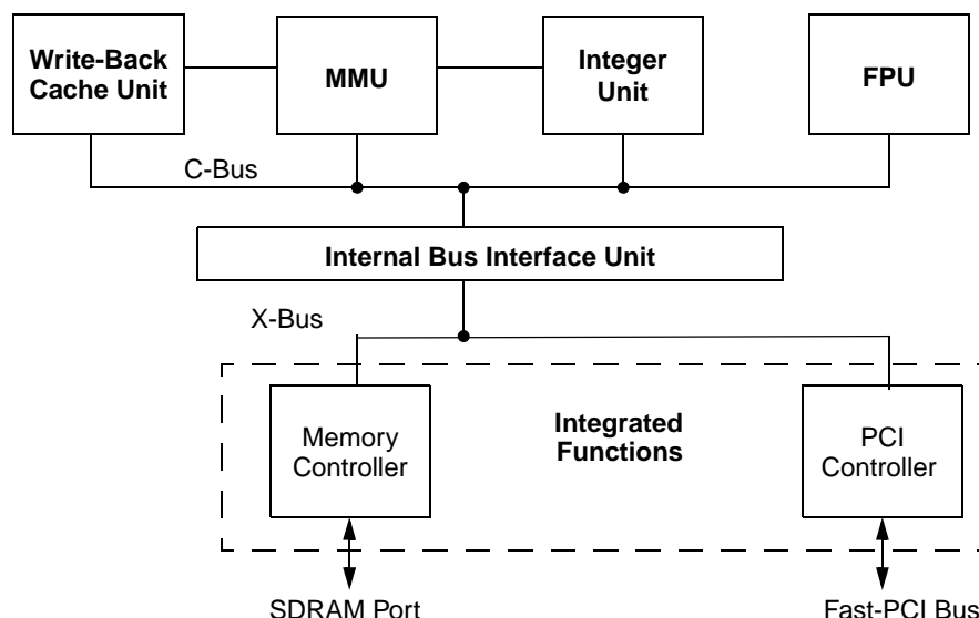
Figure 2-1. Internal Block Diagram
