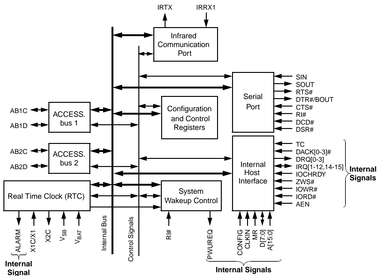
Figure 5-2. Detailed SIO Block Diagram
