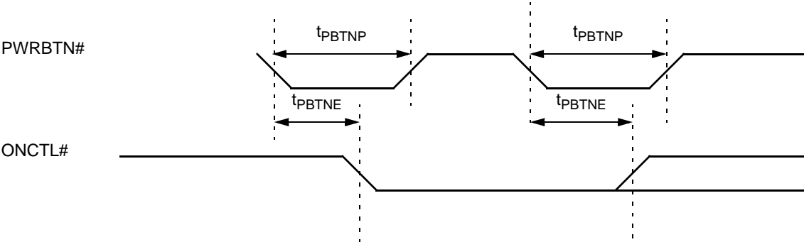
Figure 8-47. PWRBTN# Trigger and ONCTL# Timing
