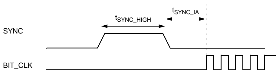
Figure 8-42. AC97 Sync Timing
