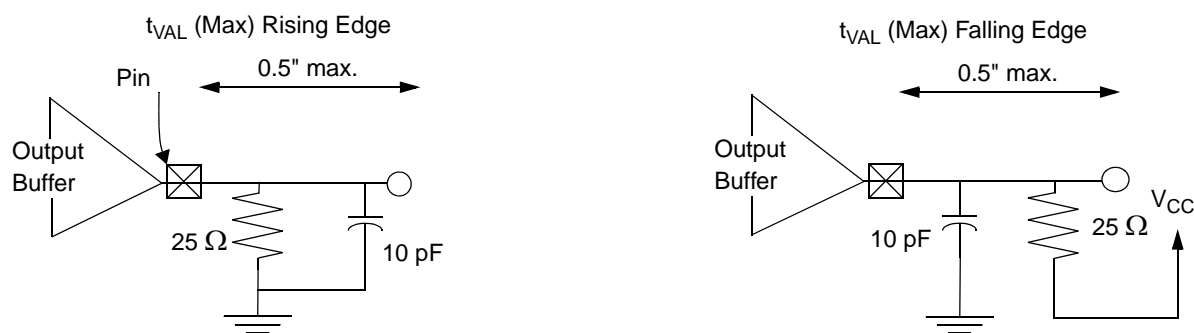
Figure 8-13. Load Circuits for Maximum Time Measurements
