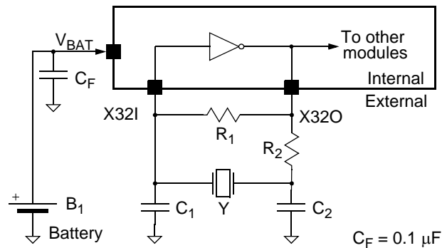
Figure 5-5. Recommended Crystal External Circuitry
