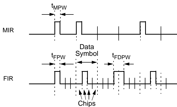
Figure 8-40. Fast IR Timing (MIR and FIR)
