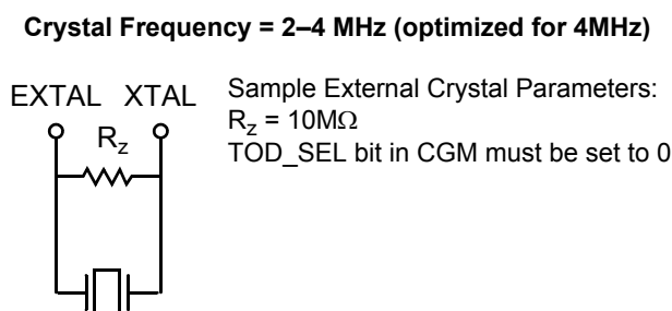
Figure 4-6 Crystal Oscillator
