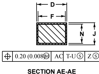
Figure 5-2 100-pin LQPF Mechanical Information
