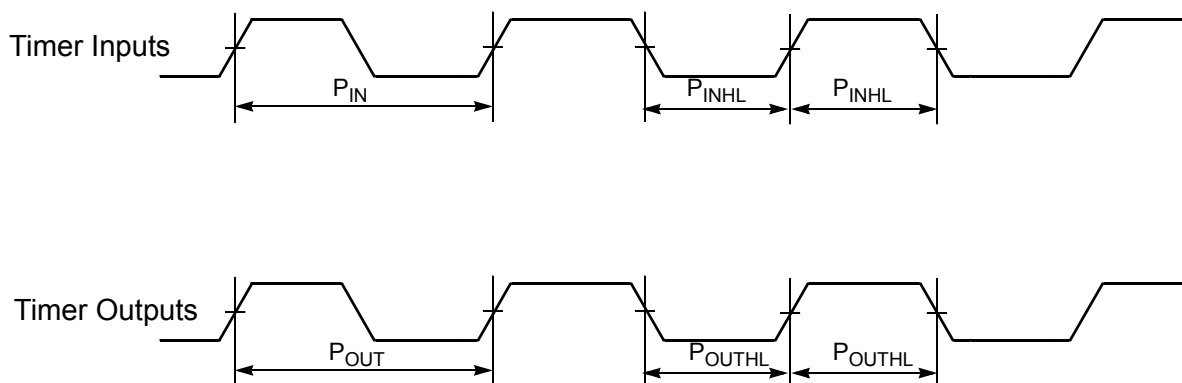
Figure 4-23 Timer Timing
