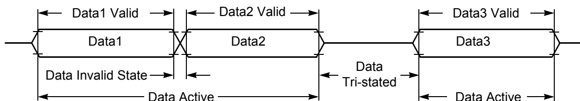
Figure 4-5 Signal State
