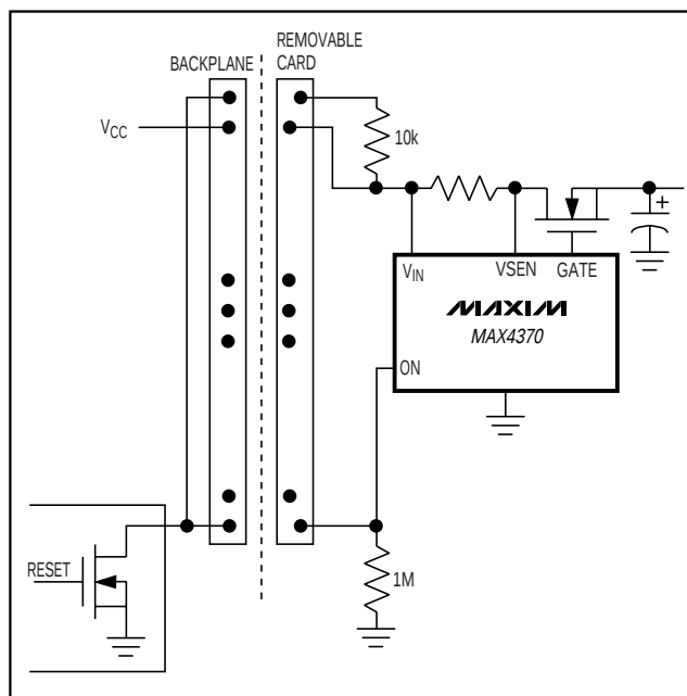
Figure 10. Fail-Safe Connector
