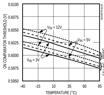
ON COMPARATOR THRESHOLD vs. TEMPERATURE
