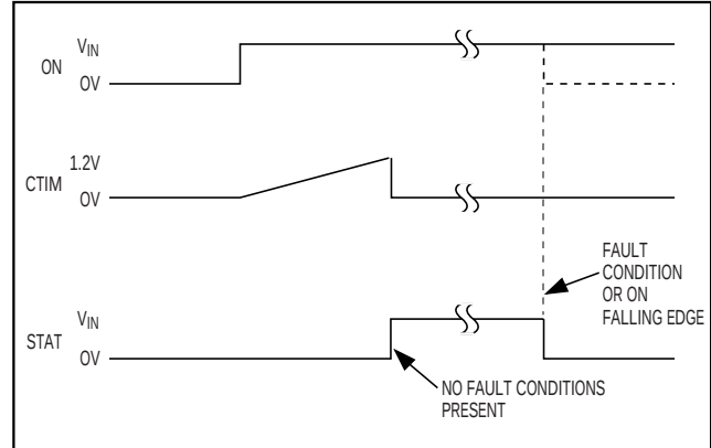
Figure 4. Status Output (STAT) Timing Diagram
