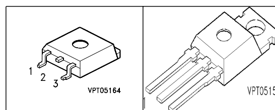
P-TO263-3-2
