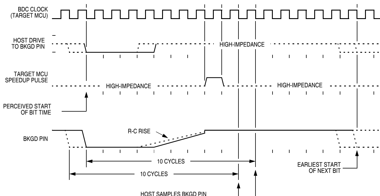
Figure 12-3. BDC Target-to-Host Serial Bit Timing (Logic 1)
