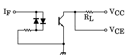
Fig.1 Switching Time Test Circuit
