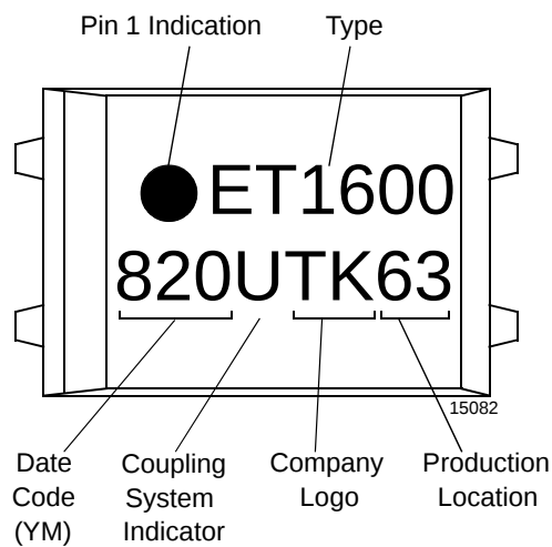
Figure 16. Marking example
