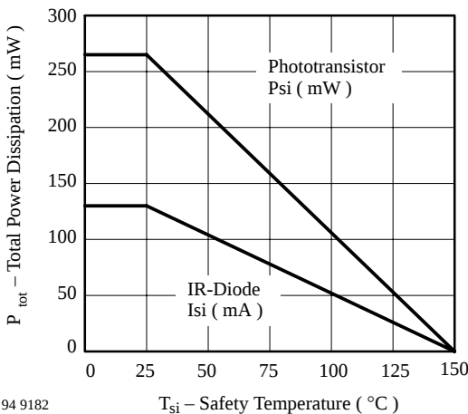
Figure 1. Derating diagram
