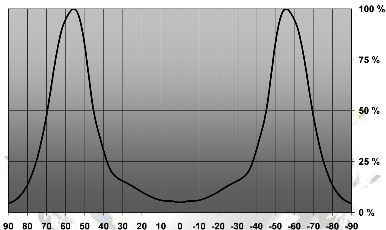
Relative Intensity of C11255_Strada-DW-XP
