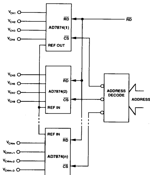
Figure 18. Multiple AD7874s in Multichannel System
