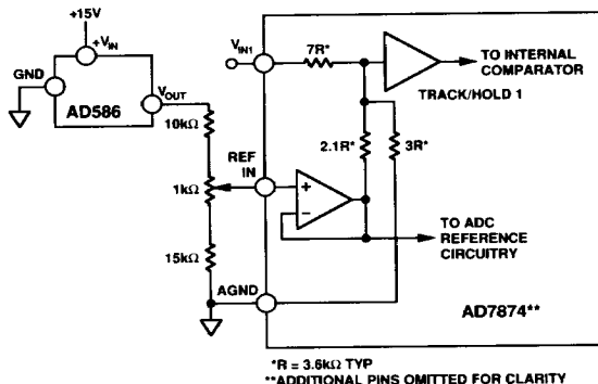
Figure 4. AD586 Driving AD7874 REF IN
