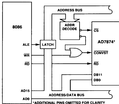
Figure 16. AD7874-8086 Interface
