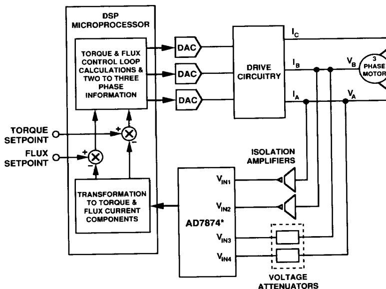
Figure 17. Vector Motor Control Using the AD7874
