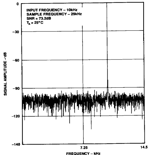
Figure 8. AD7874 FFT Plot
