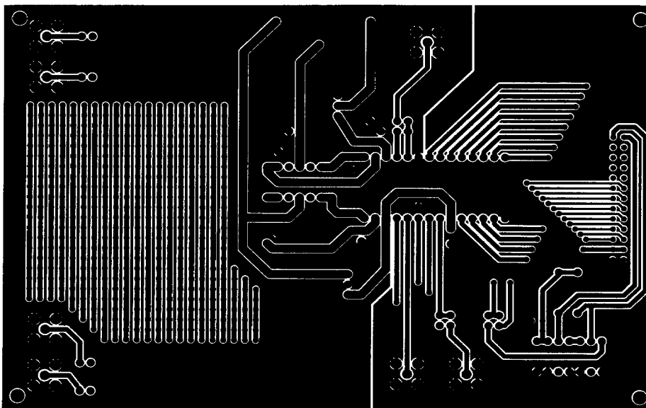
Figure 23. PCB Solder Side Layout for the Circuit of Figure 20
