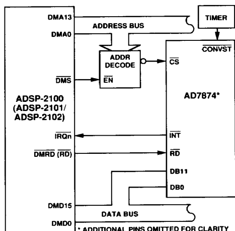
Figure 12. AD7874-ADSP-2100 Interface
