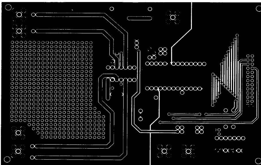
Figure 22. PCB Component Side Layout for the Circuit of Figure 20
