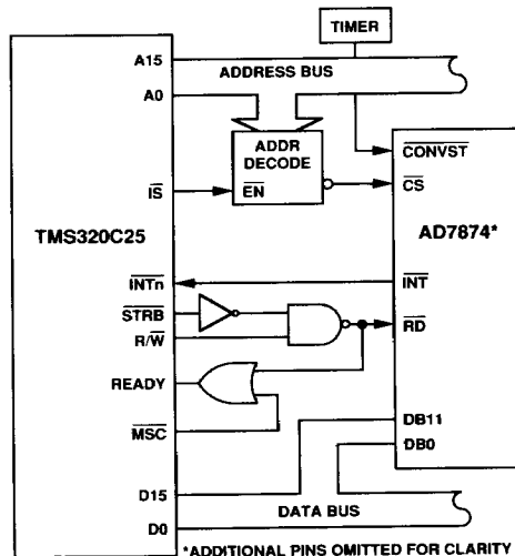
Figure 14. AD7874-TMS320C25 Interface
