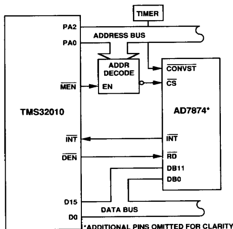
Figure 13. AD7874-TMS32010 Interface
