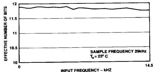
Figure 9. Effective Numbers of Bits vs. Frequency
