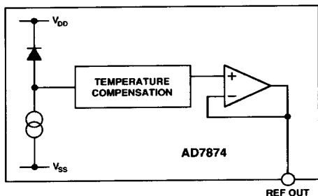
Figure 3. AD7874 Internal Reference
