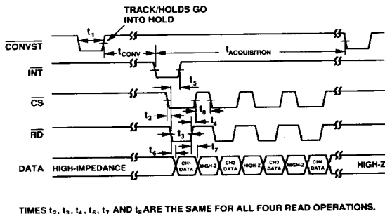
Figure 7. AD7874 Timing Diagram
