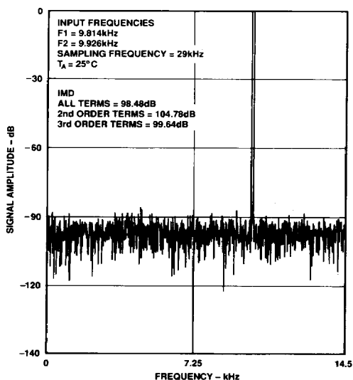
Figure 10. AD7874 IMD Plot
