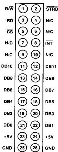
Figure 19. SKT8, IDC Connector Pinout
