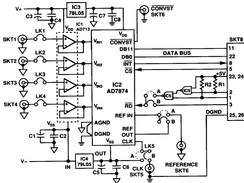
Figure 20. Data Acquisition Circuit Using the AD7874
