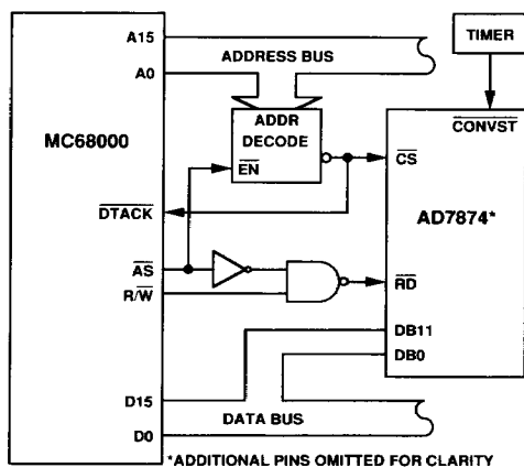
Figure 15. AD7874-MC68000 Interface
