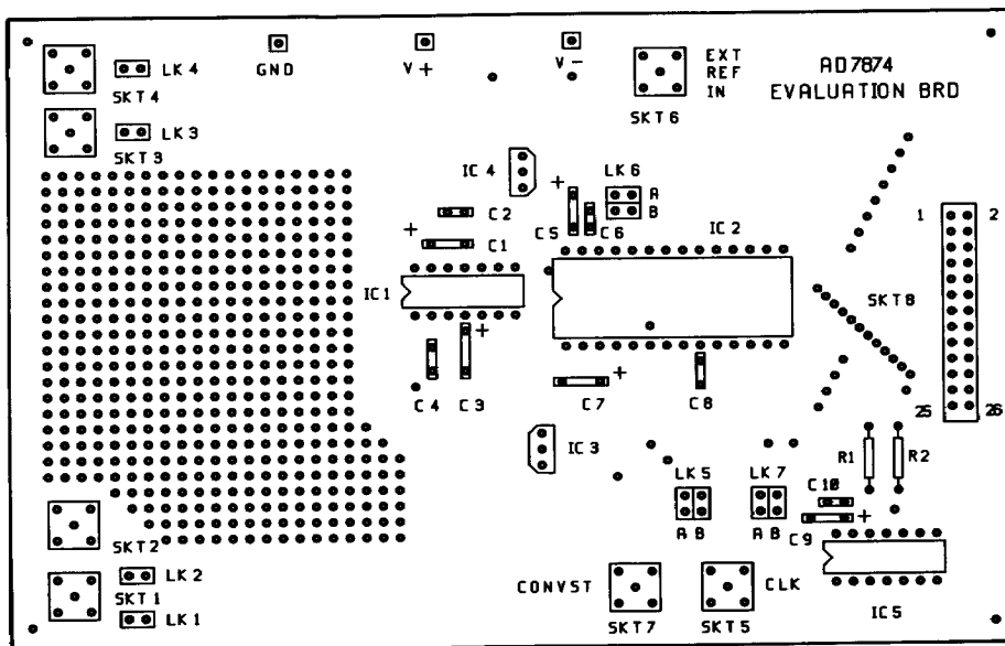
Figure 21. PCB Silkscreen for Figure 20
