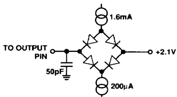
Figure 2. Load Circuit for Bus Relinquish Time
