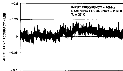
Figure 11. AD7874 AC INL Plot
